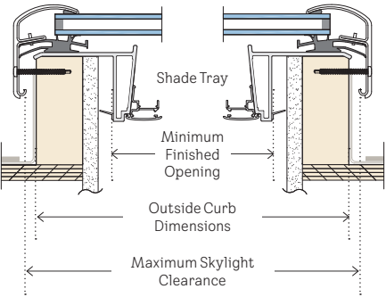
Flashed curb at minimum range constraint will result in 3/4" gap between skylight frame and flashed curb. Flashed curb at maximum range constraint will result in 1/8" gap between skylight frame and flashed curb.
