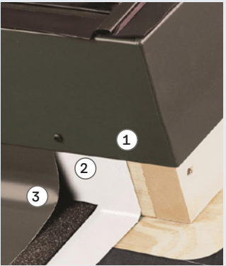
Curb-Mounted
